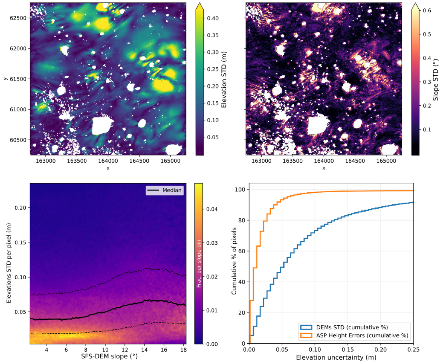
Figure 8. from Stefano Bertone et al 2026 Planet. Sci. J. 7 doi:10.3847/PSJ/ae5b70 https://dx.doi.org/10.3847/PSJ/ae5b70 © 2026. The Author(s). Published by the American Astronomical Society.
