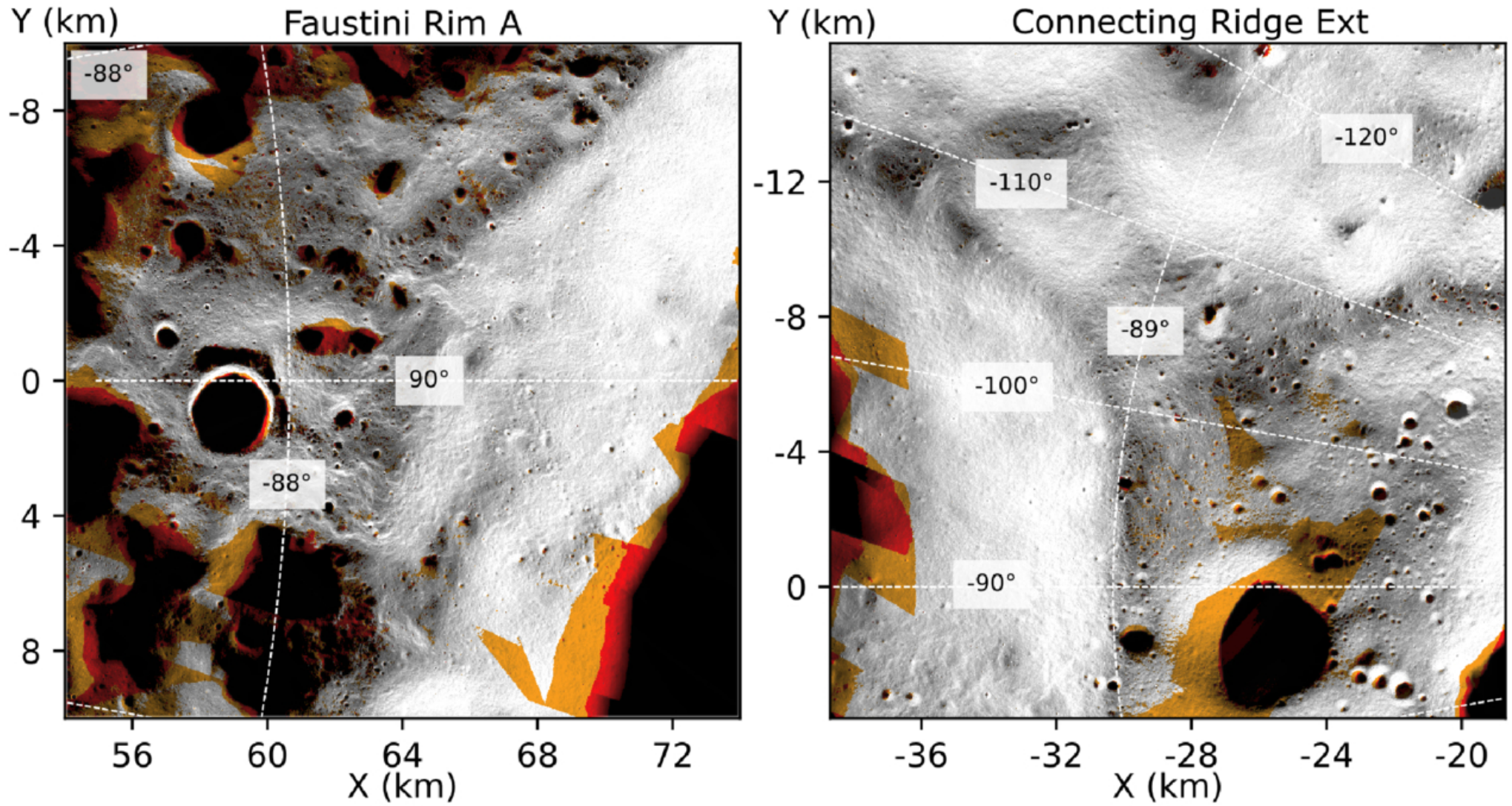
Figure 6. from Stefano Bertone et al 2026 Planet. Sci. J. 7 doi:10.3847/PSJ/ae5b70 https://dx.doi.org/10.3847/PSJ/ae5b70 © 2026. The Author(s). Published by the American Astronomical Society.
