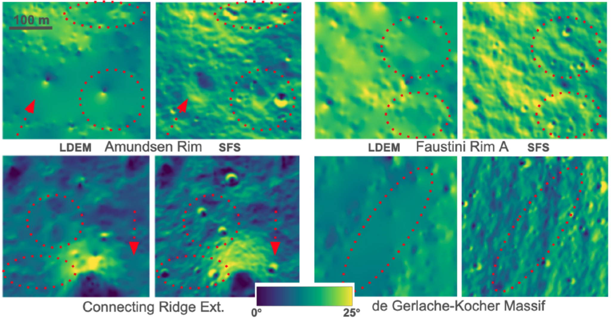
Figure 2. from Stefano Bertone et al 2026 Planet. Sci. J. 7 doi:10.3847/PSJ/ae5b70 https://dx.doi.org/10.3847/PSJ/ae5b70 © 2026. The Author(s). Published by the American Astronomical Society.
