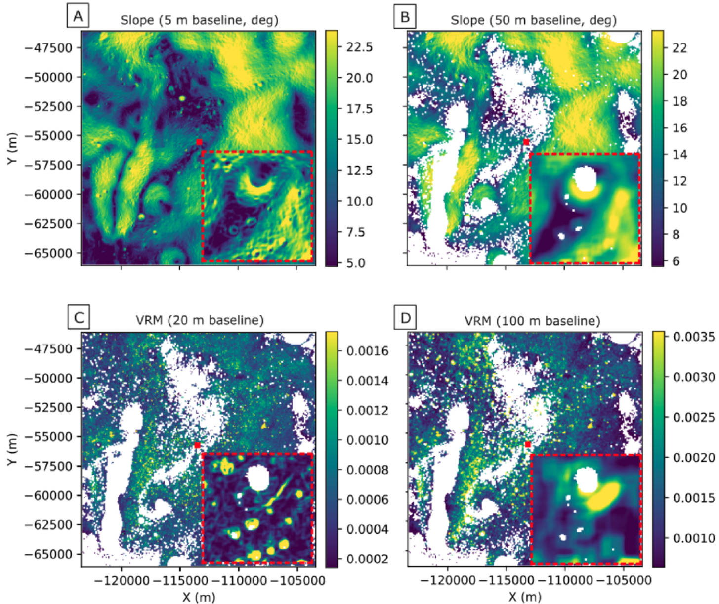
Figure 19. from Stefano Bertone et al 2026 Planet. Sci. J. 7 doi:10.3847/PSJ/ae5b70 https://dx.doi.org/10.3847/PSJ/ae5b70 © 2026. The Author(s). Published by the American Astronomical Society.
