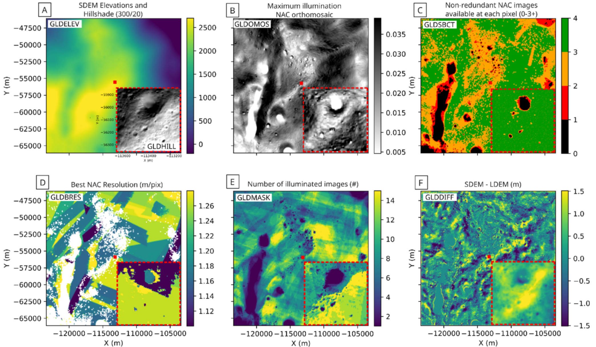
Figure 18. from Stefano Bertone et al 2026 Planet. Sci. J. 7 doi:10.3847/PSJ/ae5b70 https://dx.doi.org/10.3847/PSJ/ae5b70 © 2026. The Author(s). Published by the American Astronomical Society.
