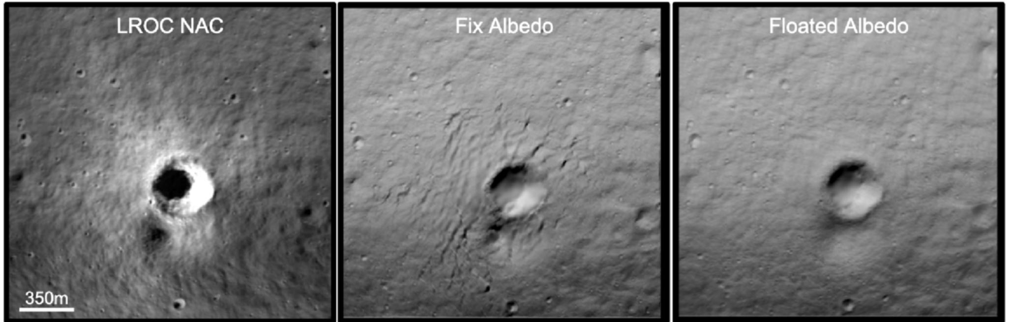
Figure 17. from Stefano Bertone et al 2026 Planet. Sci. J. 7 doi:10.3847/PSJ/ae5b70 https://dx.doi.org/10.3847/PSJ/ae5b70 © 2026. The Author(s). Published by the American Astronomical Society.
