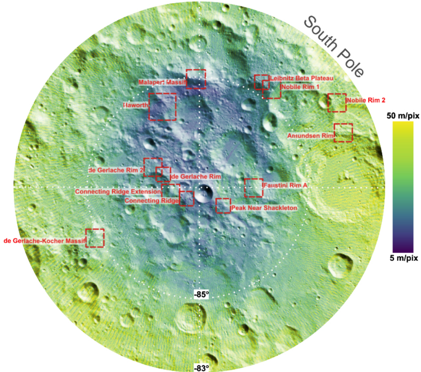
Figure 1. from Stefano Bertone et al 2026 Planet. Sci. J. 7 doi:10.3847/PSJ/ae5b70 https://dx.doi.org/10.3847/PSJ/ae5b70 © 2026. The Author(s). Published by the American Astronomical Society.
