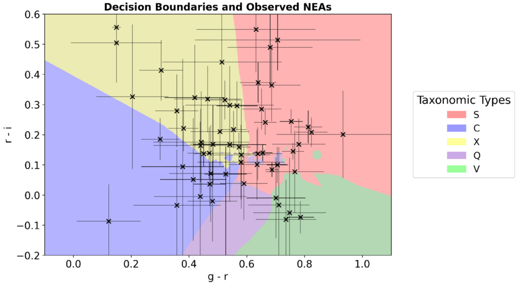
Figure 4. from Thobekile S. Ngwane et al 2026 Planet. Sci. J. 7 doi:10.3847/PSJ/ae5b69 https://dx.doi.org/10.3847/PSJ/ae5b69 © 2026. The Author(s). Published by the American Astronomical Society.
