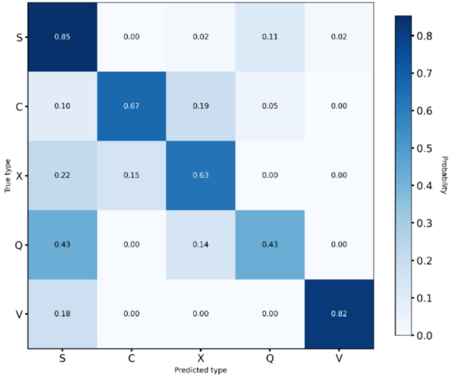
Figure 3. from Thobekile S. Ngwane et al 2026 Planet. Sci. J. 7 doi:10.3847/PSJ/ae5b69 https://dx.doi.org/10.3847/PSJ/ae5b69 © 2026. The Author(s). Published by the American Astronomical Society.
