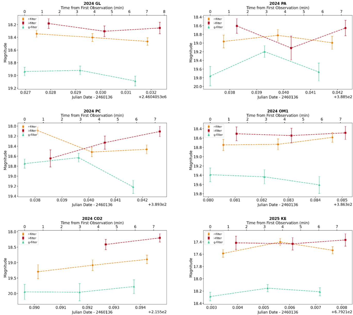
Figure 2. from Thobekile S. Ngwane et al 2026 Planet. Sci. J. 7 doi:10.3847/PSJ/ae5b69 https://dx.doi.org/10.3847/PSJ/ae5b69 © 2026. The Author(s). Published by the American Astronomical Society.
