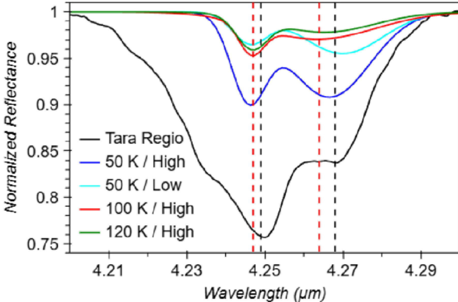
Figure 6. from Ashma Pandya et al 2026 Planet. Sci. J. 7 doi:10.3847/PSJ/ae595b https://dx.doi.org/10.3847/PSJ/ae595b © 2026. The Author(s). Published by the American Astronomical Society.
