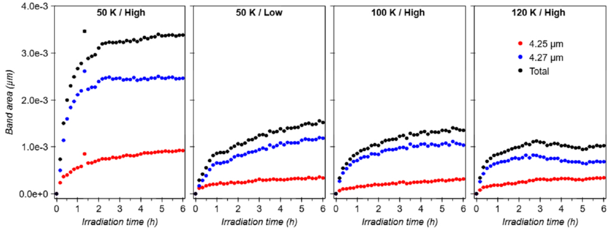
Figure 3. from Ashma Pandya et al 2026 Planet. Sci. J. 7 doi:10.3847/PSJ/ae595b https://dx.doi.org/10.3847/PSJ/ae595b © 2026. The Author(s). Published by the American Astronomical Society.
