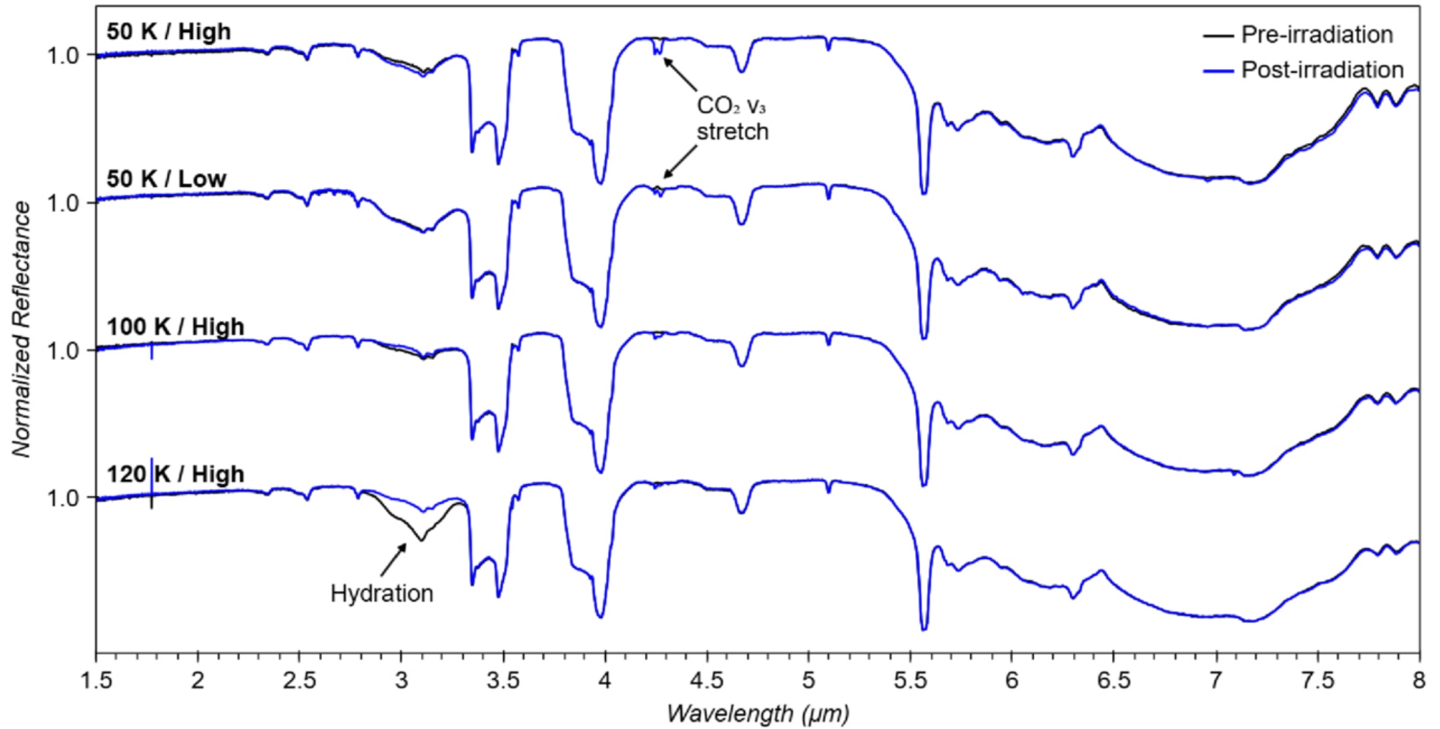
Figure 1. from Ashma Pandya et al 2026 Planet. Sci. J. 7 doi:10.3847/PSJ/ae595b https://dx.doi.org/10.3847/PSJ/ae595b © 2026. The Author(s). Published by the American Astronomical Society.
