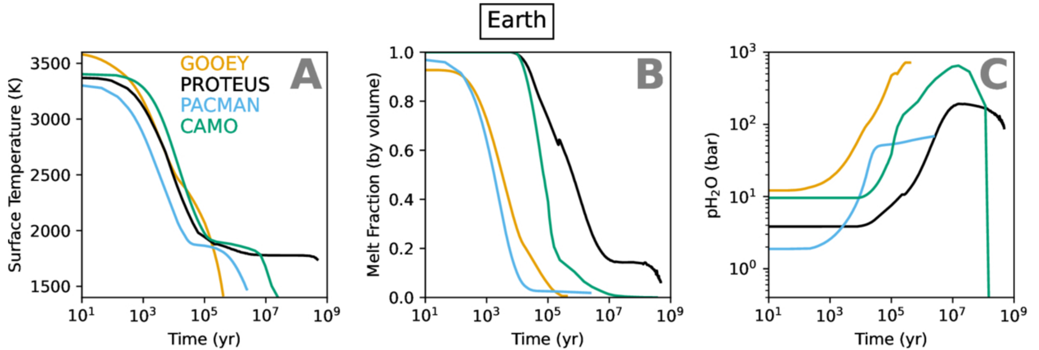
Figure 2. from Tim Lichtenberg et al 2026 Planet. Sci. J. 7 doi:10.3847/PSJ/ae593b https://dx.doi.org/10.3847/PSJ/ae593b © 2026. The Author(s). Published by the American Astronomical Society.
