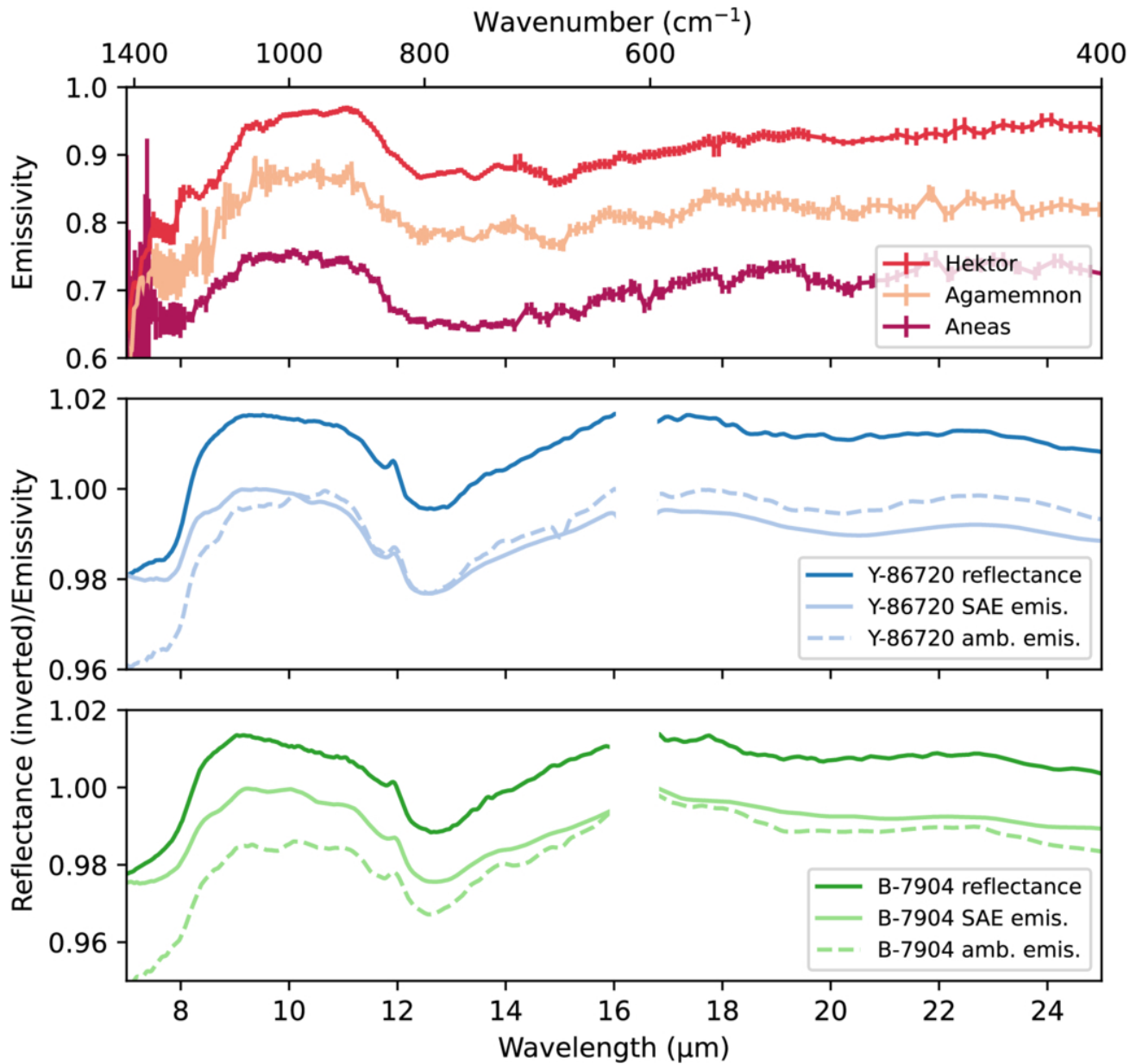
Figure 3. from Helena C. Bates et al 2026 Planet. Sci. J. 7 doi:10.3847/PSJ/ae5931 https://dx.doi.org/10.3847/PSJ/ae5931 © 2026. The Author(s). Published by the American Astronomical Society.
