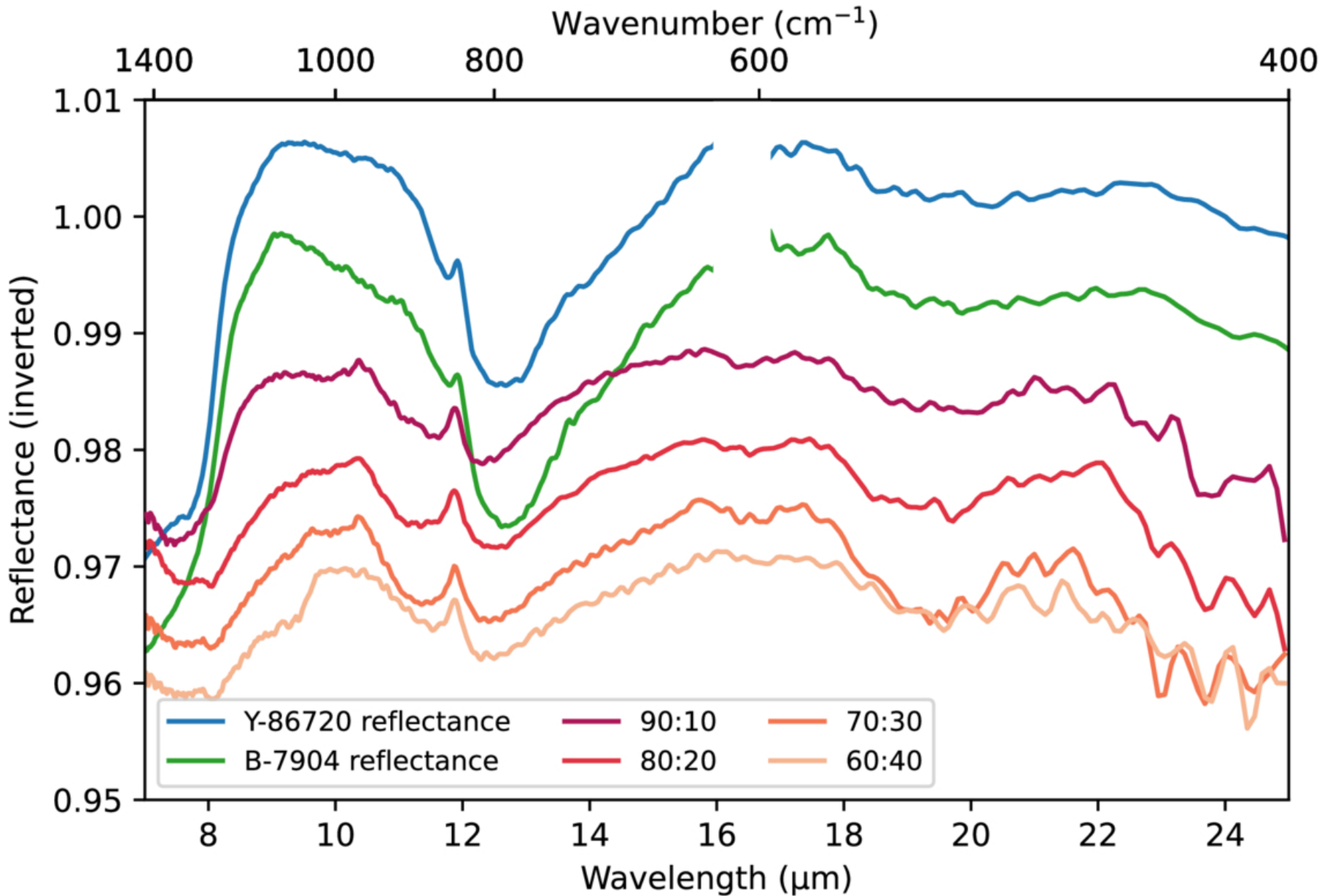
Figure 2. from Helena C. Bates et al 2026 Planet. Sci. J. 7 doi:10.3847/PSJ/ae5931 https://dx.doi.org/10.3847/PSJ/ae5931 © 2026. The Author(s). Published by the American Astronomical Society.
