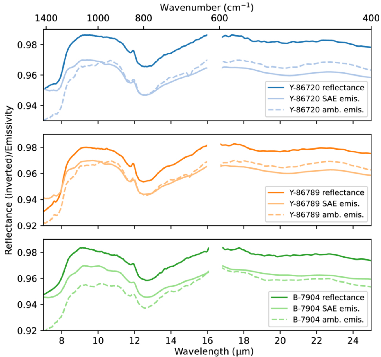
Figure 1. from Helena C. Bates et al 2026 Planet. Sci. J. 7 doi:10.3847/PSJ/ae5931 https://dx.doi.org/10.3847/PSJ/ae5931 © 2026. The Author(s). Published by the American Astronomical Society.
