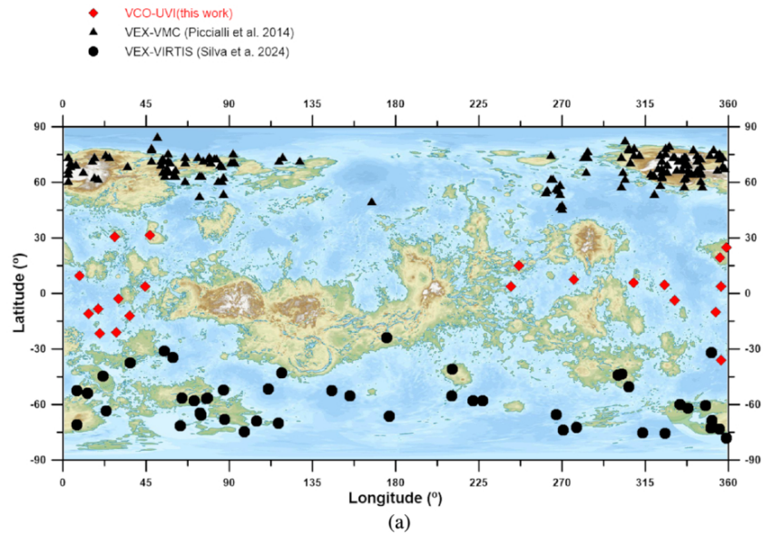
Figure 9. from Daniela Espadinha et al 2026 Planet. Sci. J. 7 doi:10.3847/PSJ/ae592e https://dx.doi.org/10.3847/PSJ/ae592e © 2026. The Author(s). Published by the American Astronomical Society.
