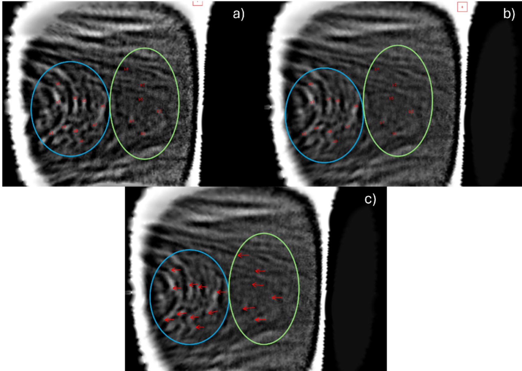
Figure 8. from Daniela Espadinha et al 2026 Planet. Sci. J. 7 doi:10.3847/PSJ/ae592e https://dx.doi.org/10.3847/PSJ/ae592e © 2026. The Author(s). Published by the American Astronomical Society.
