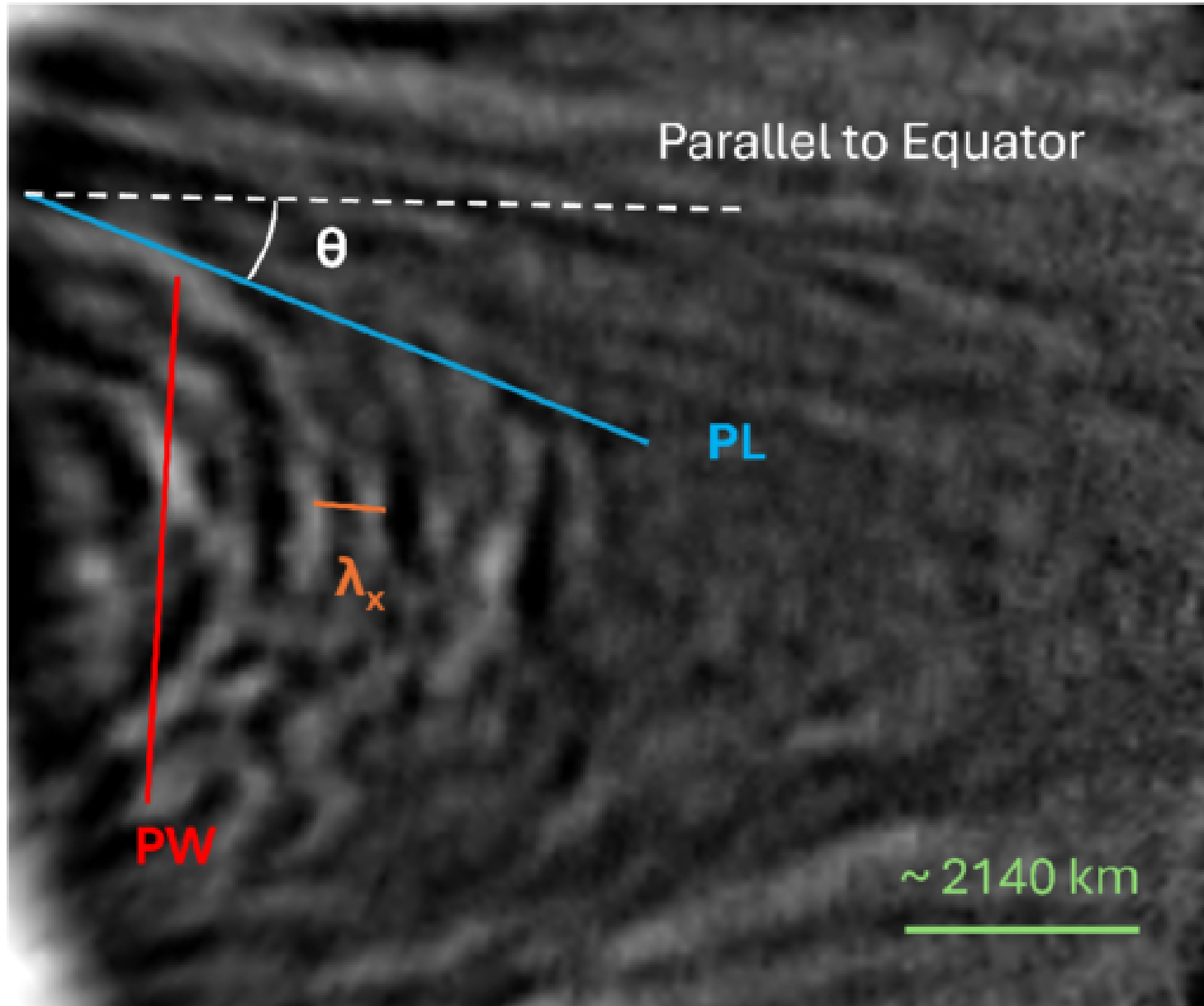
Figure 7. from Daniela Espadinha et al 2026 Planet. Sci. J. 7 doi:10.3847/PSJ/ae592e https://dx.doi.org/10.3847/PSJ/ae592e © 2026. The Author(s). Published by the American Astronomical Society.
