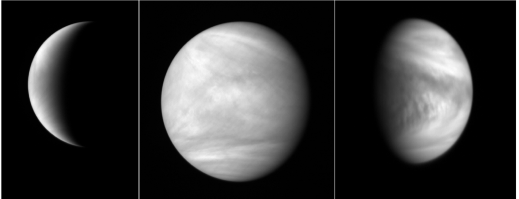
Figure 5. from Daniela Espadinha et al 2026 Planet. Sci. J. 7 doi:10.3847/PSJ/ae592e https://dx.doi.org/10.3847/PSJ/ae592e © 2026. The Author(s). Published by the American Astronomical Society.
