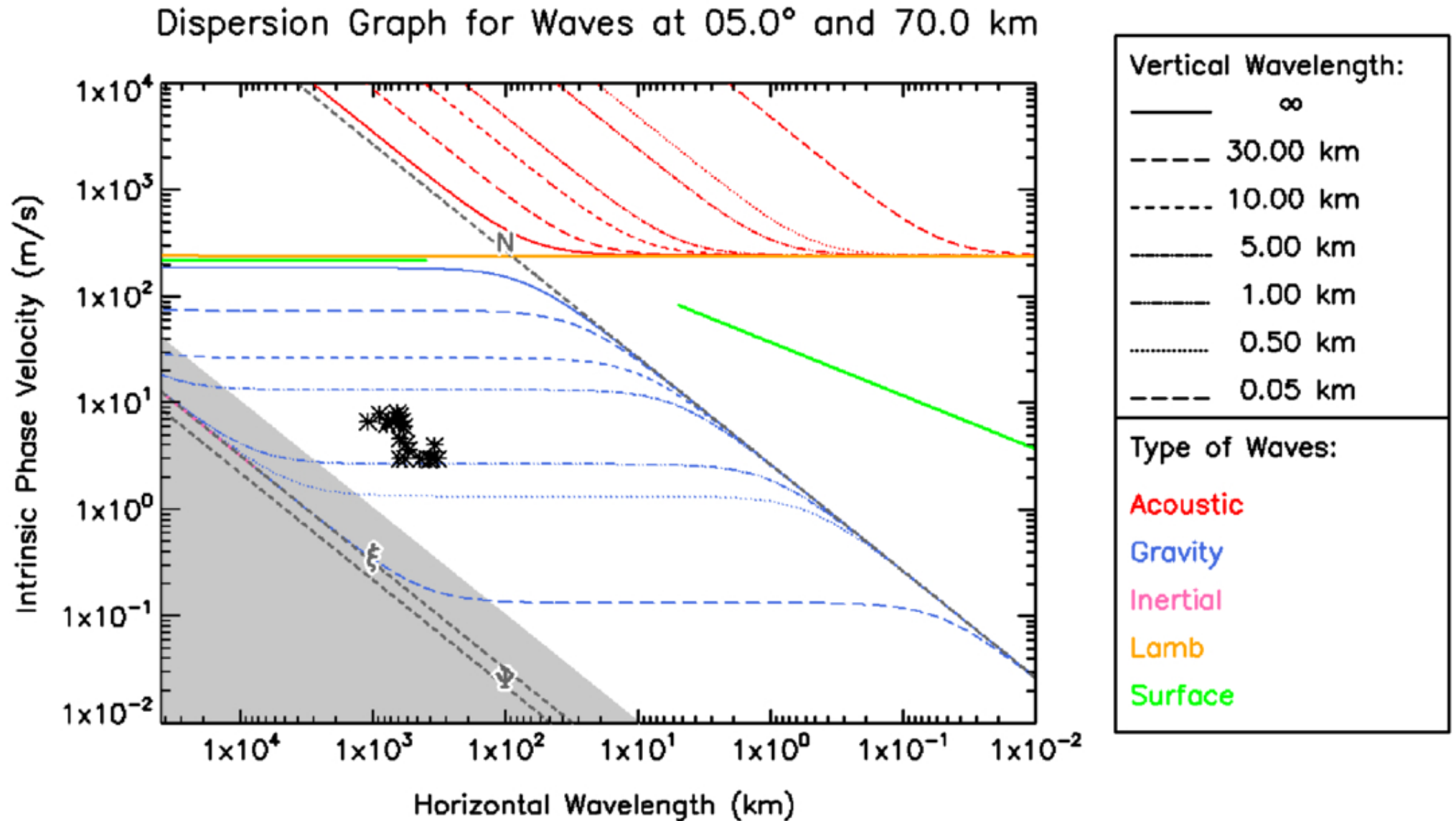
Figure 18. from Daniela Espadinha et al 2026 Planet. Sci. J. 7 doi:10.3847/PSJ/ae592e https://dx.doi.org/10.3847/PSJ/ae592e © 2026. The Author(s). Published by the American Astronomical Society.
