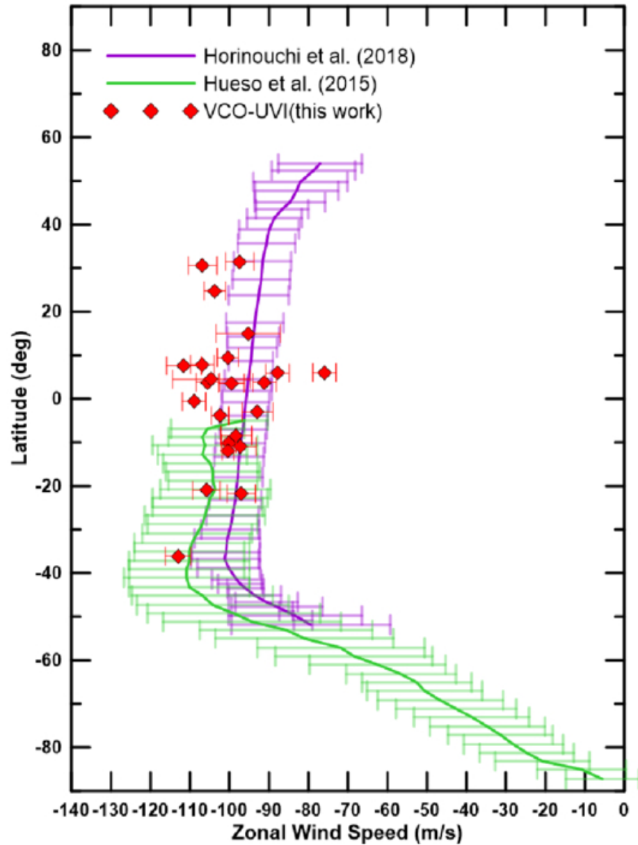
Figure 13. from Daniela Espadinha et al 2026 Planet. Sci. J. 7 doi:10.3847/PSJ/ae592e https://dx.doi.org/10.3847/PSJ/ae592e © 2026. The Author(s). Published by the American Astronomical Society.
