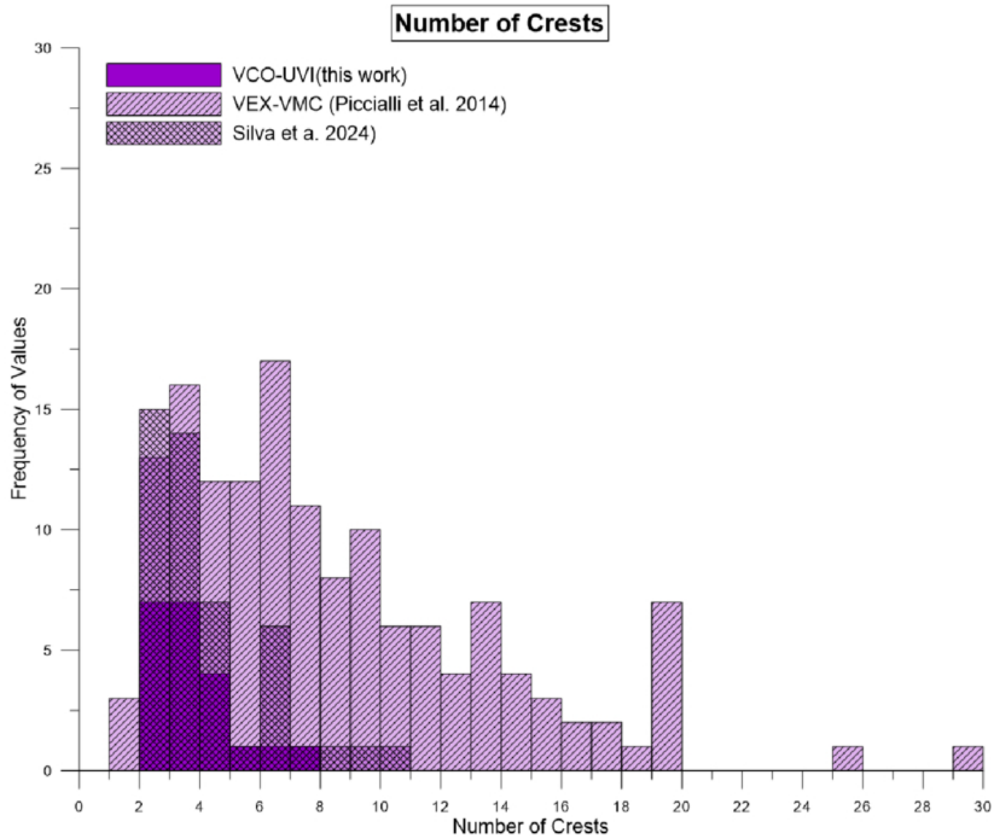
Figure 12. from Daniela Espadinha et al 2026 Planet. Sci. J. 7 doi:10.3847/PSJ/ae592e https://dx.doi.org/10.3847/PSJ/ae592e © 2026. The Author(s). Published by the American Astronomical Society.
