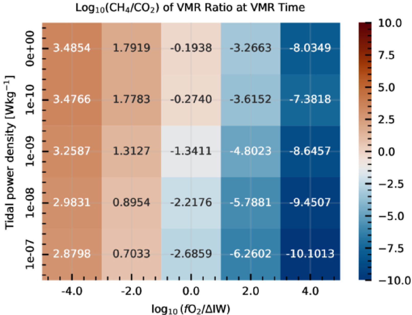
Figure 9. from Marijn R. van Dijk et al 2026 Planet. Sci. J. 7 doi:10.3847/PSJ/ae5928 https://dx.doi.org/10.3847/PSJ/ae5928 © 2026. The Author(s). Published by the American Astronomical Society.
