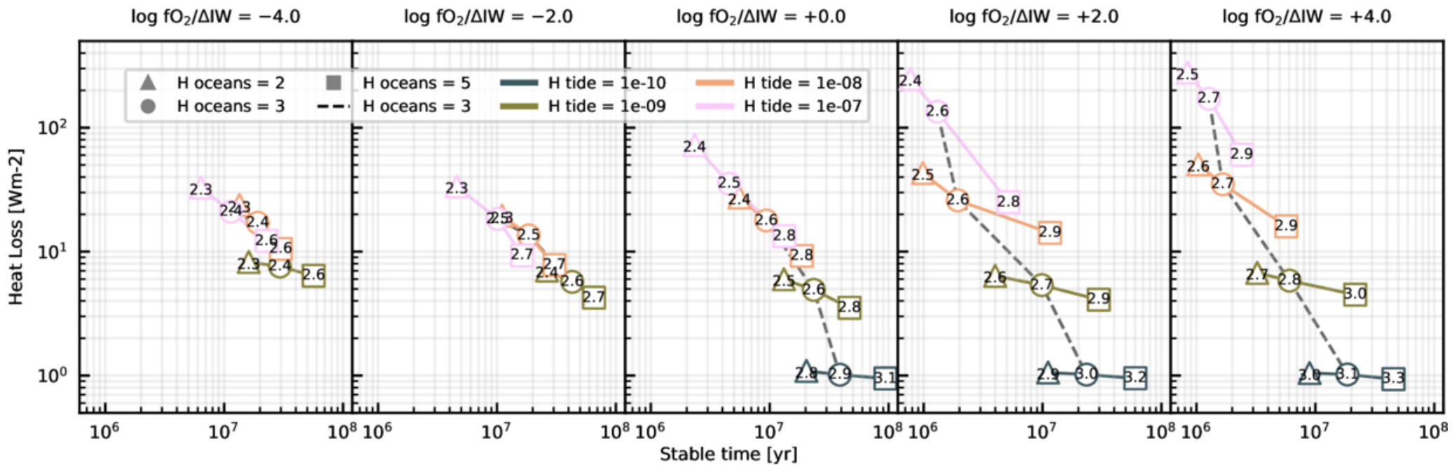
Figure 6. from Marijn R. van Dijk et al 2026 Planet. Sci. J. 7 doi:10.3847/PSJ/ae5928 https://dx.doi.org/10.3847/PSJ/ae5928 © 2026. The Author(s). Published by the American Astronomical Society.
