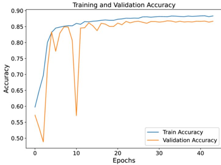
(a) Training and validation accuracy vs. epochs.
