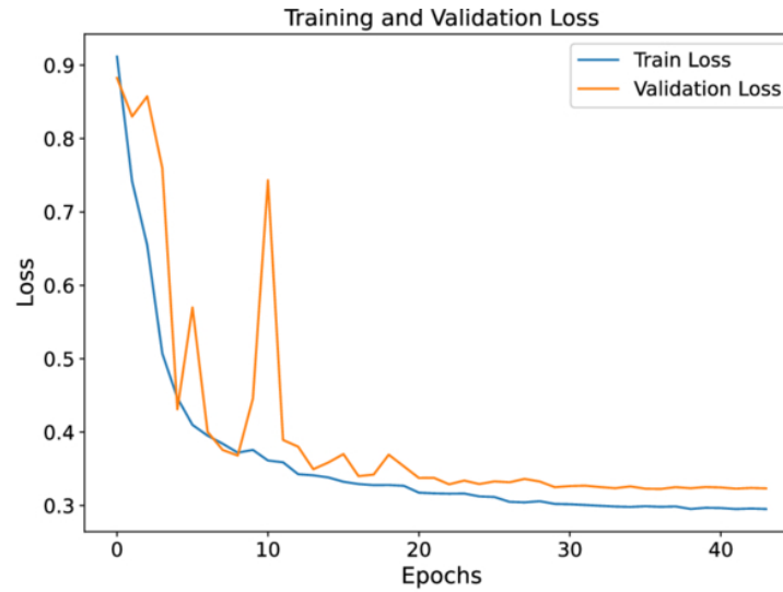
(b) Training and validation loss vs. epochs.
