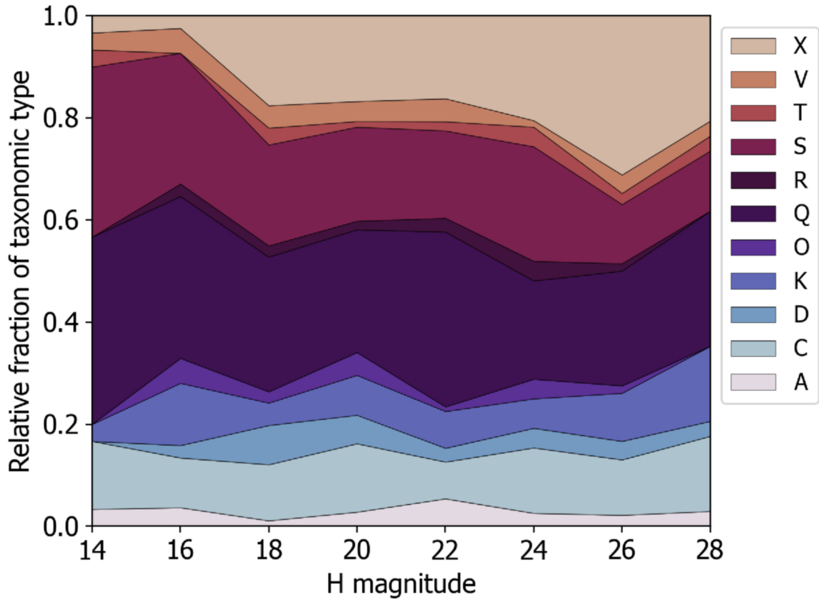
Figure 9. from Nicholas Moskovitz et al 2026 Planet. Sci. J. 7 doi:10.3847/PSJ/ae5642 https://dx.doi.org/10.3847/PSJ/ae5642 © 2026. The Author(s). Published by the American Astronomical Society.
