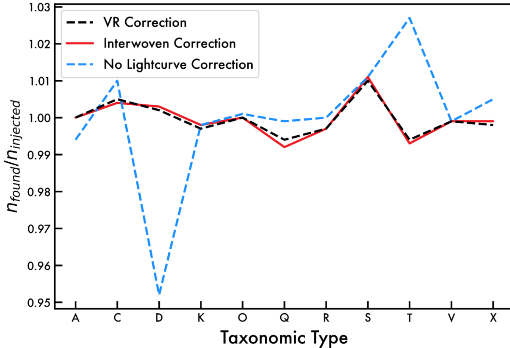
Figure 8. from Nicholas Moskovitz et al 2026 Planet. Sci. J. 7 doi:10.3847/PSJ/ae5642 https://dx.doi.org/10.3847/PSJ/ae5642 © 2026. The Author(s). Published by the American Astronomical Society.
