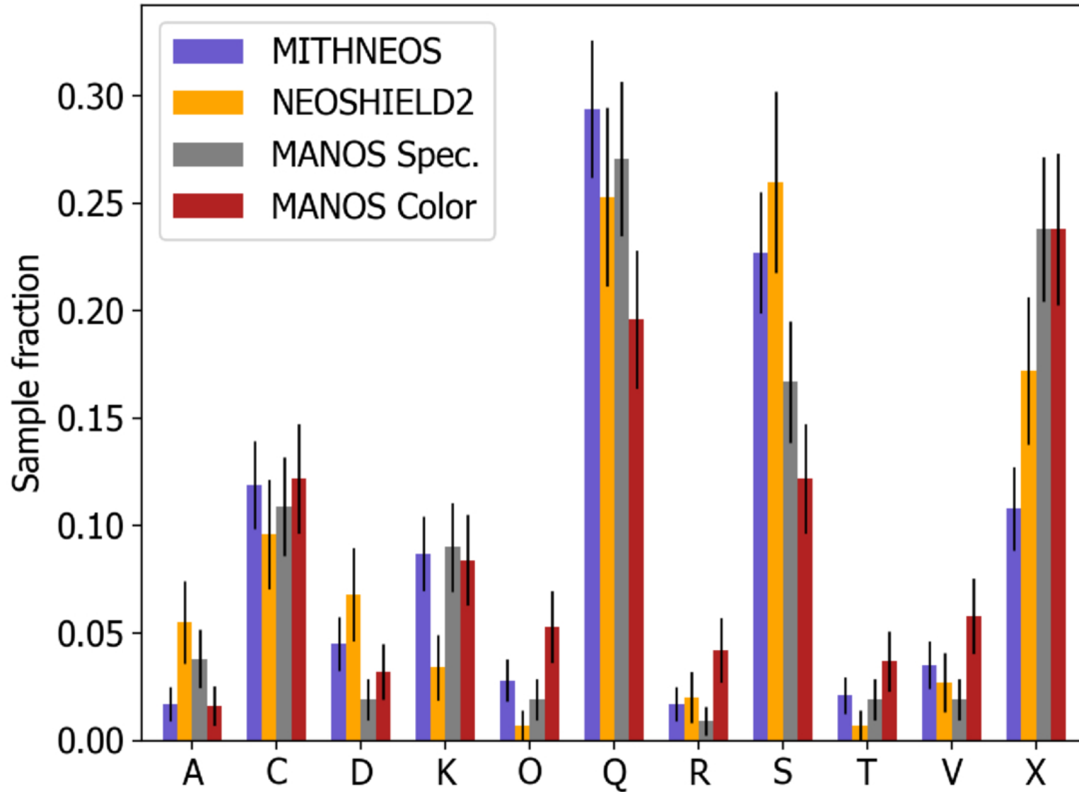
Figure 5. from Nicholas Moskovitz et al 2026 Planet. Sci. J. 7 doi:10.3847/PSJ/ae5642 https://dx.doi.org/10.3847/PSJ/ae5642 © 2026. The Author(s). Published by the American Astronomical Society.
