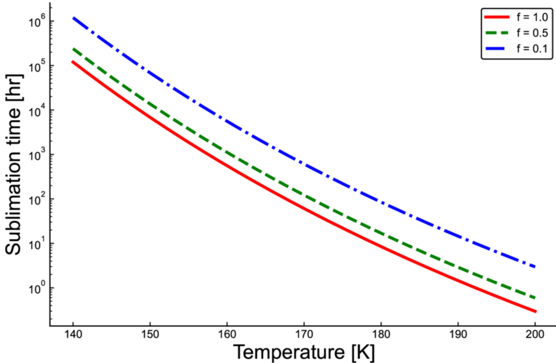
Figure 5. from Jun Takeshita et al 2026 Planet. Sci. J. 7 doi:10.3847/PSJ/ae548e https://dx.doi.org/10.3847/PSJ/ae548e © 2026. The Author(s). Published by the American Astronomical Society.
