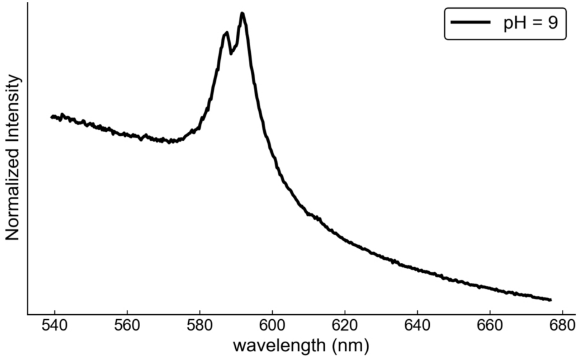
Figure 4. from Jun Takeshita et al 2026 Planet. Sci. J. 7 doi:10.3847/PSJ/ae548e https://dx.doi.org/10.3847/PSJ/ae548e © 2026. The Author(s). Published by the American Astronomical Society.
