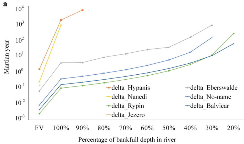
Figure 5. from Yaowen Luo et al 2026 Planet. Sci. J. 7 doi:10.3847/PSJ/ae53dd https://dx.doi.org/10.3847/PSJ/ae53dd © 2026. The Author(s). Published by the American Astronomical Society.
