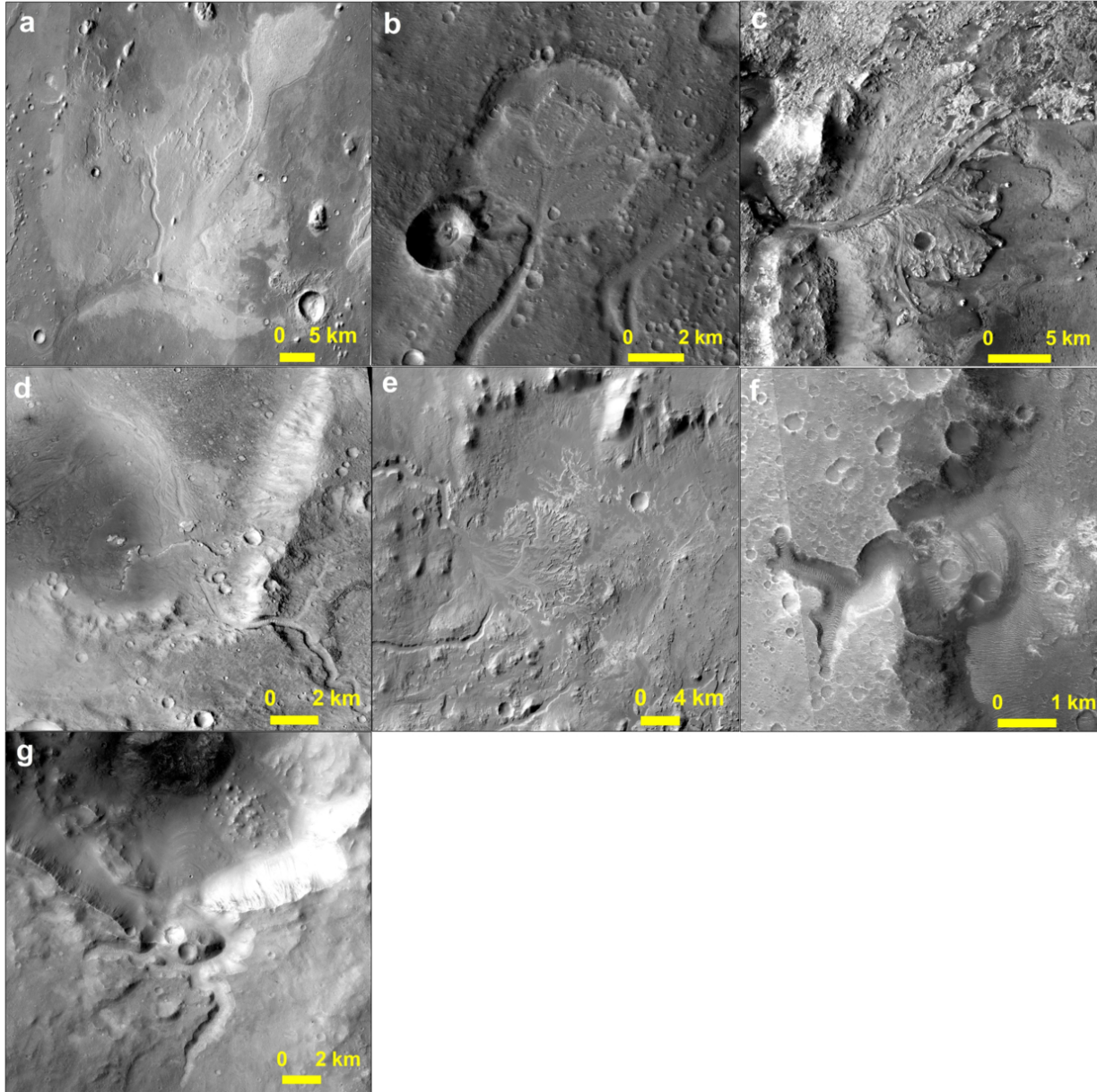
Figure 1. from Yaowen Luo et al 2026 Planet. Sci. J. 7 doi:10.3847/PSJ/ae53dd https://dx.doi.org/10.3847/PSJ/ae53dd © 2026. The Author(s). Published by the American Astronomical Society.
