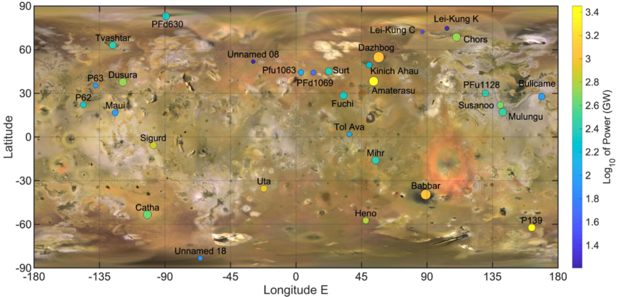
Figure 4. from Alessandro Mura et al 2026 Planet. Sci. J. 7 doi:10.3847/PSJ/ae52ee https://dx.doi.org/10.3847/PSJ/ae52ee © 2026. The Author(s). Published by the American Astronomical Society.
