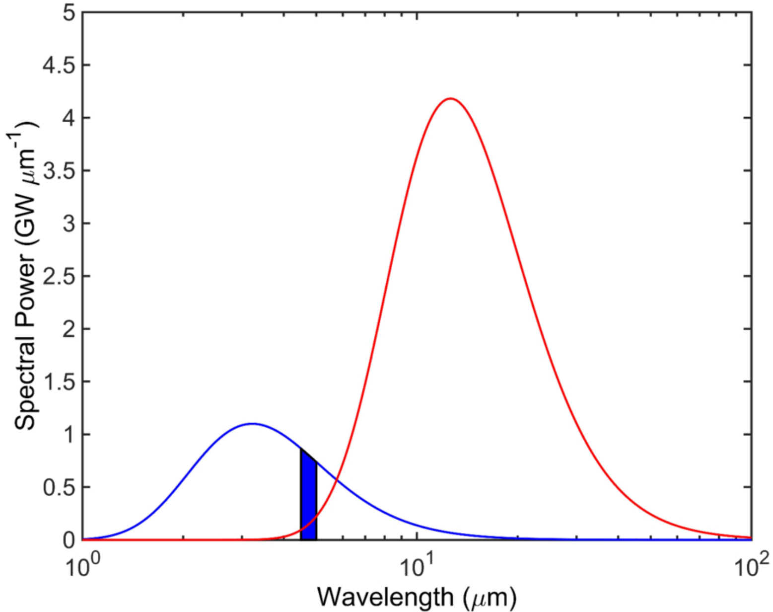
Figure 3. from Alessandro Mura et al 2026 Planet. Sci. J. 7 doi:10.3847/PSJ/ae52ee https://dx.doi.org/10.3847/PSJ/ae52ee © 2026. The Author(s). Published by the American Astronomical Society.
