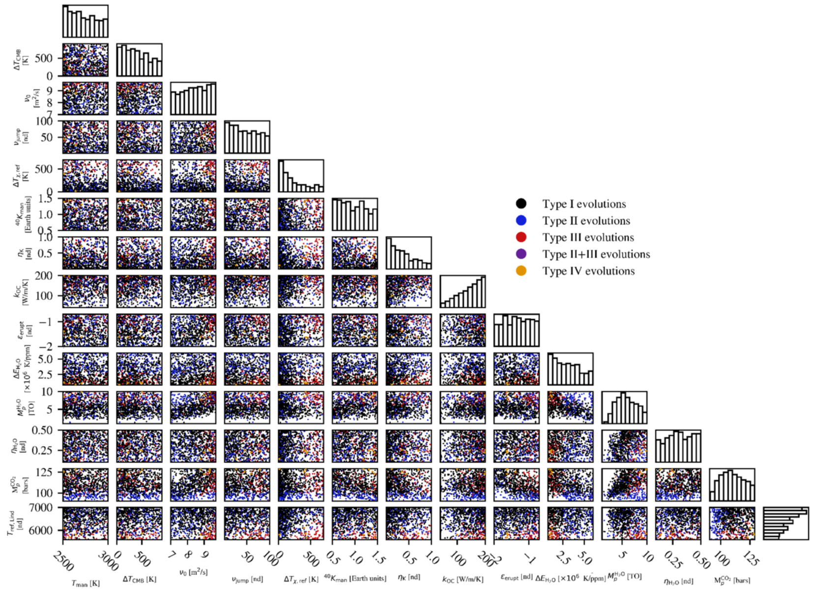
Figure 8. from Rodolfo Garcia et al 2026 Planet. Sci. J. 7 doi:10.3847/PSJ/ae5248 https://dx.doi.org/10.3847/PSJ/ae5248 © 2026. The Author(s). Published by the American Astronomical Society.
