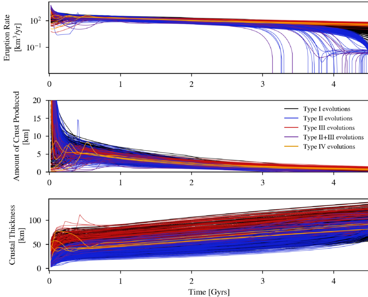
Figure 25. from Rodolfo Garcia et al 2026 Planet. Sci. J. 7 doi:10.3847/PSJ/ae5248 https://dx.doi.org/10.3847/PSJ/ae5248 © 2026. The Author(s). Published by the American Astronomical Society.
