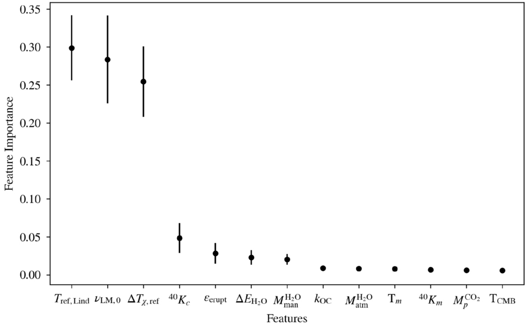
Figure 18. from Rodolfo Garcia et al 2026 Planet. Sci. J. 7 doi:10.3847/PSJ/ae5248 https://dx.doi.org/10.3847/PSJ/ae5248 © 2026. The Author(s). Published by the American Astronomical Society.
