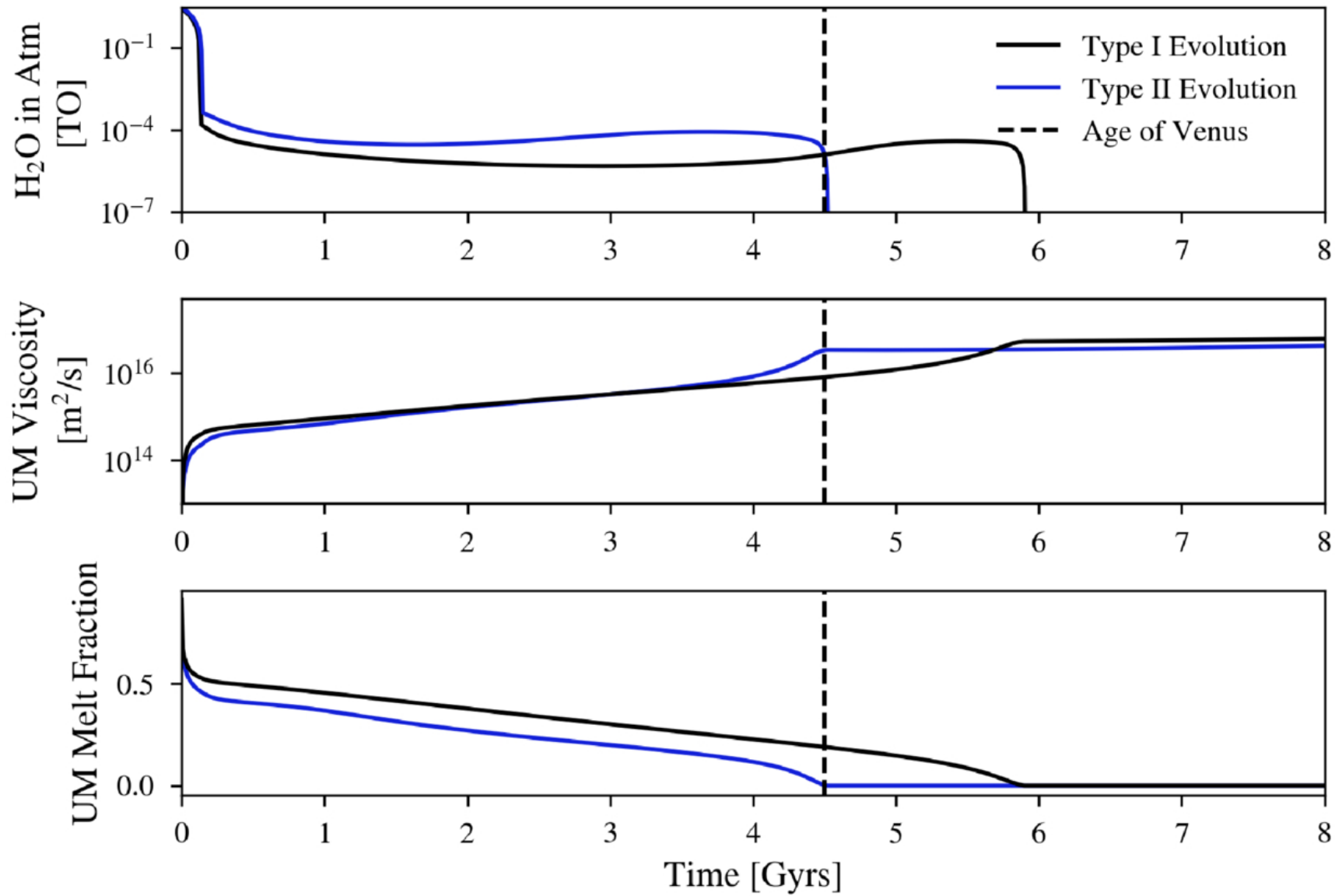
Figure 16. from Rodolfo Garcia et al 2026 Planet. Sci. J. 7 doi:10.3847/PSJ/ae5248 https://dx.doi.org/10.3847/PSJ/ae5248 © 2026. The Author(s). Published by the American Astronomical Society.
