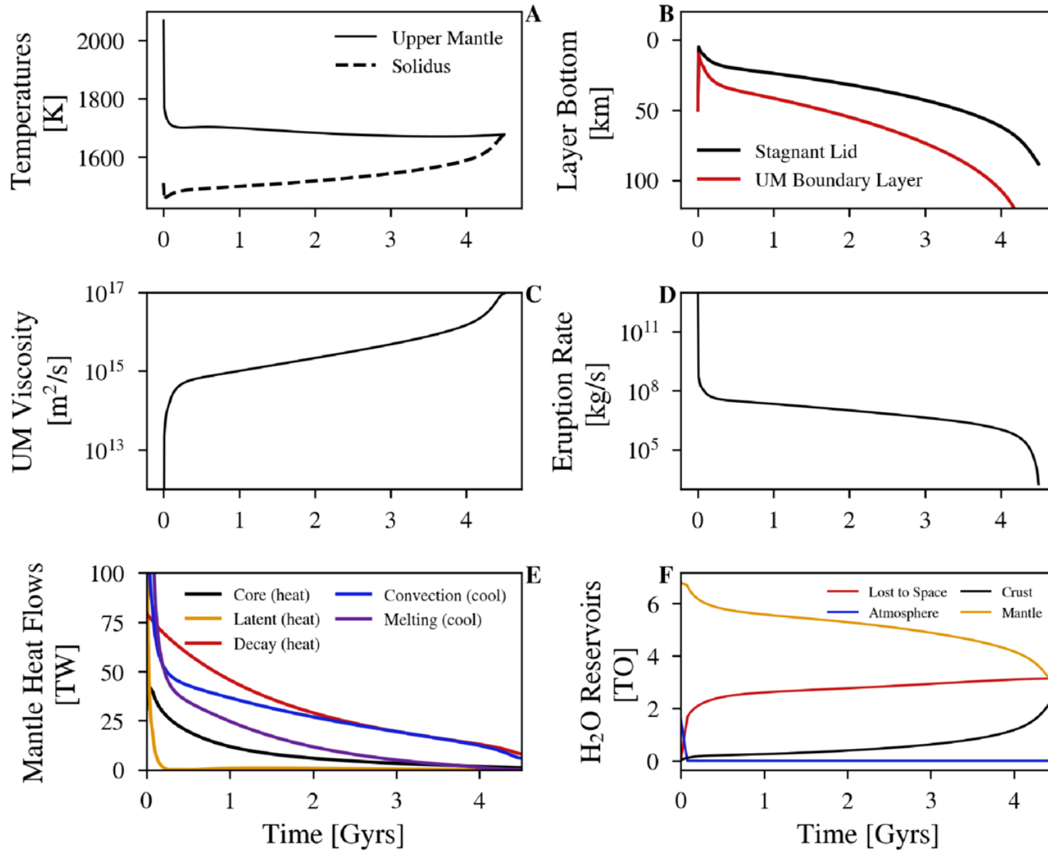
Figure 11. from Rodolfo Garcia et al 2026 Planet. Sci. J. 7 doi:10.3847/PSJ/ae5248 https://dx.doi.org/10.3847/PSJ/ae5248 © 2026. The Author(s). Published by the American Astronomical Society.
