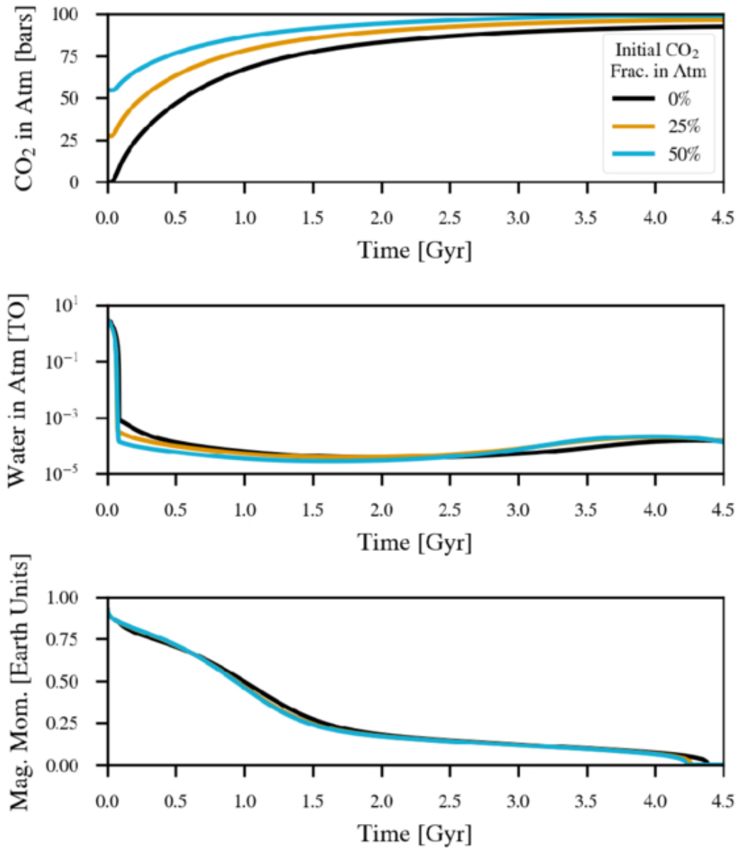
Figure 10. from Rodolfo Garcia et al 2026 Planet. Sci. J. 7 doi:10.3847/PSJ/ae5248 https://dx.doi.org/10.3847/PSJ/ae5248 © 2026. The Author(s). Published by the American Astronomical Society.
