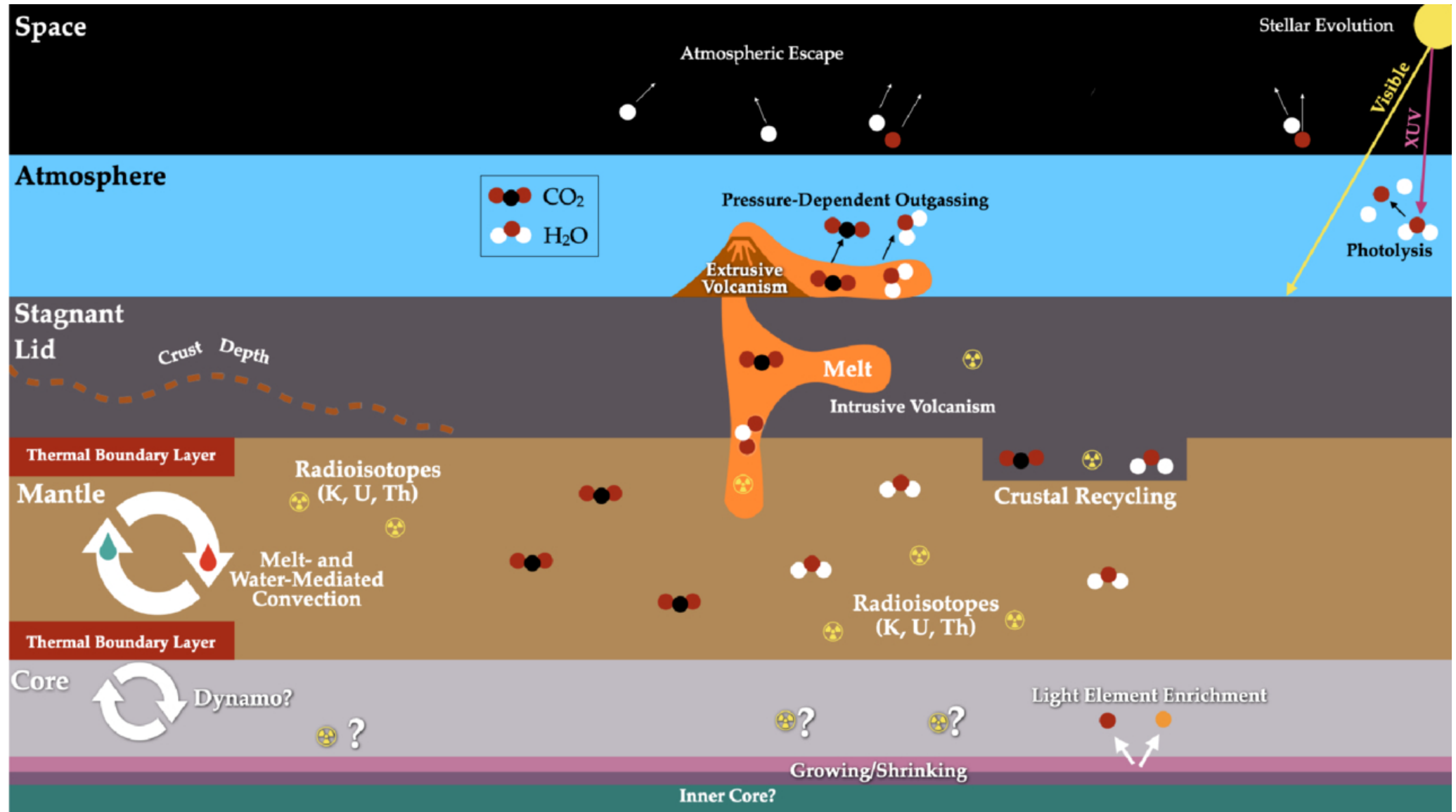
Figure 1. from Rodolfo Garcia et al 2026 Planet. Sci. J. 7 doi:10.3847/PSJ/ae5248 https://dx.doi.org/10.3847/PSJ/ae5248 © 2026. The Author(s). Published by the American Astronomical Society.
