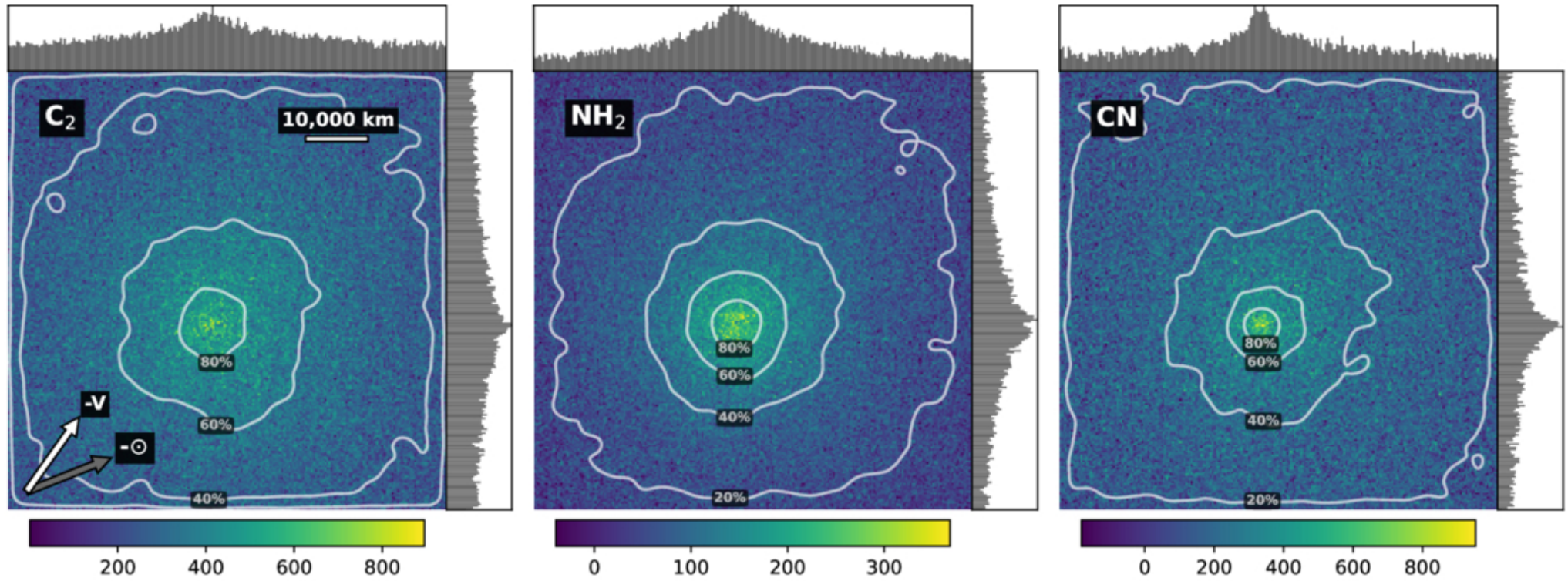
Figure 8. from Sophie E. Deam et al 2026 Planet. Sci. J. 7 doi:10.3847/PSJ/ae5244 https://dx.doi.org/10.3847/PSJ/ae5244 © 2026. The Author(s). Published by the American Astronomical Society.
