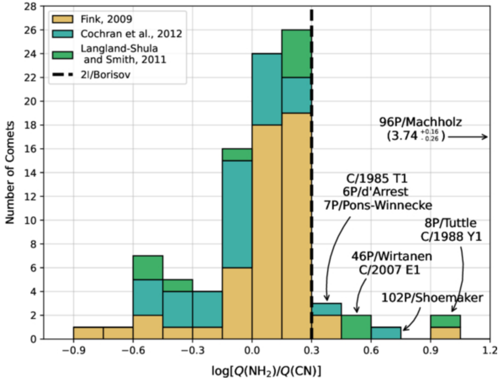
Figure 10. from Sophie E. Deam et al 2026 Planet. Sci. J. 7 doi:10.3847/PSJ/ae5244 https://dx.doi.org/10.3847/PSJ/ae5244 © 2026. The Author(s). Published by the American Astronomical Society.
