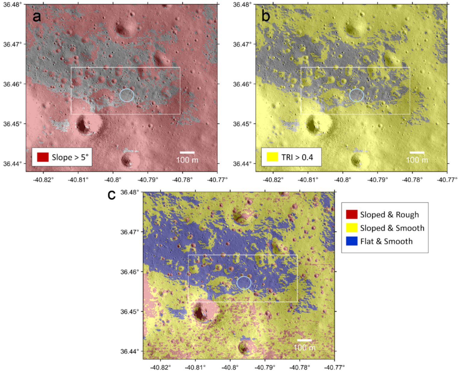
Figure 9. from Jean-Pierre Williams et al 2026 Planet. Sci. J. 7 doi:10.3847/PSJ/ae523b https://dx.doi.org/10.3847/PSJ/ae523b © 2026. The Author(s). Published by the American Astronomical Society.
