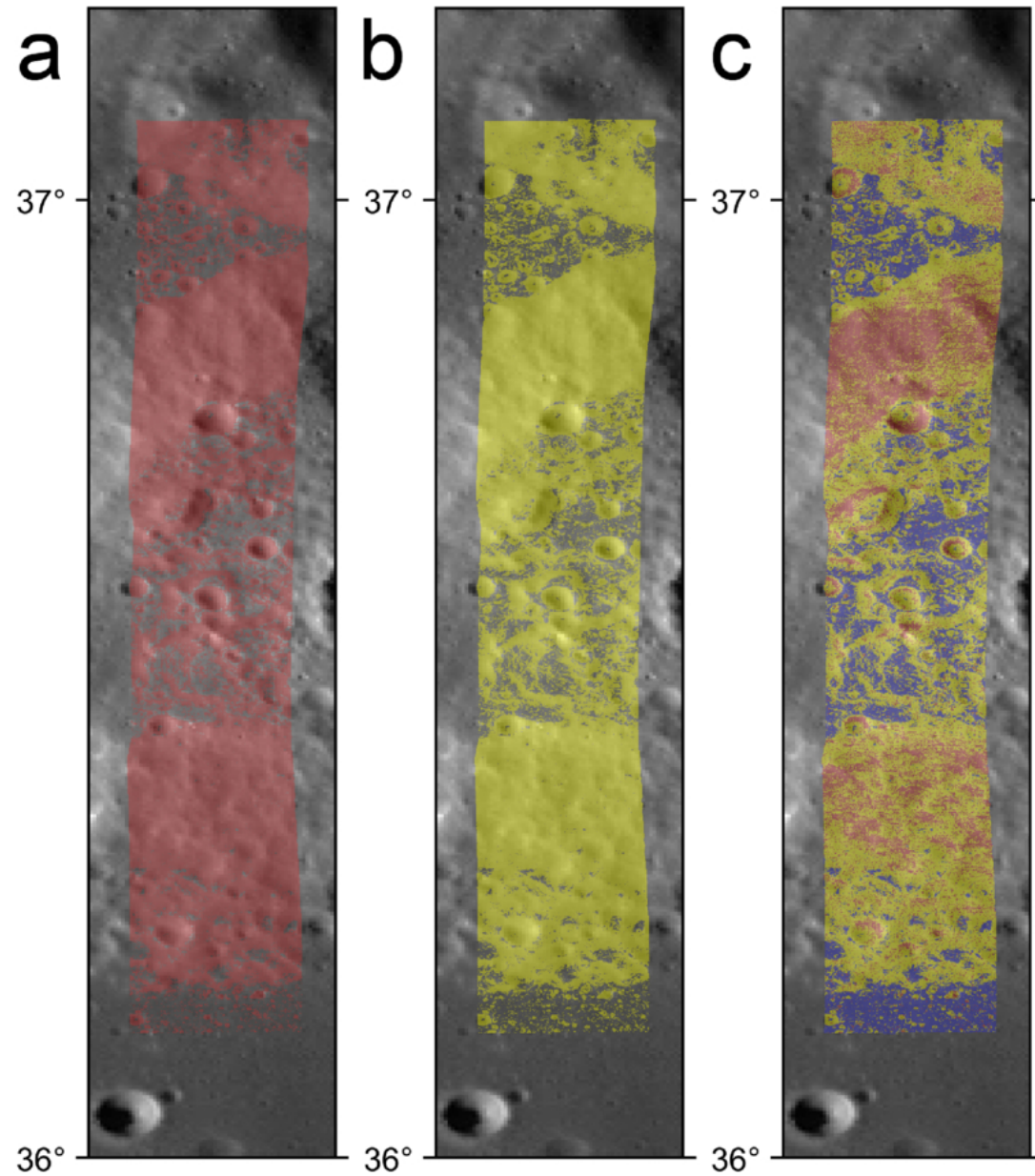
Figure 8. from Jean-Pierre Williams et al 2026 Planet. Sci. J. 7 doi:10.3847/PSJ/ae523b https://dx.doi.org/10.3847/PSJ/ae523b © 2026. The Author(s). Published by the American Astronomical Society.
