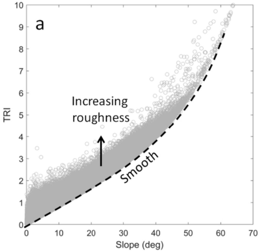
Figure 5. from Jean-Pierre Williams et al 2026 Planet. Sci. J. 7 doi:10.3847/PSJ/ae523b https://dx.doi.org/10.3847/PSJ/ae523b © 2026. The Author(s). Published by the American Astronomical Society.
