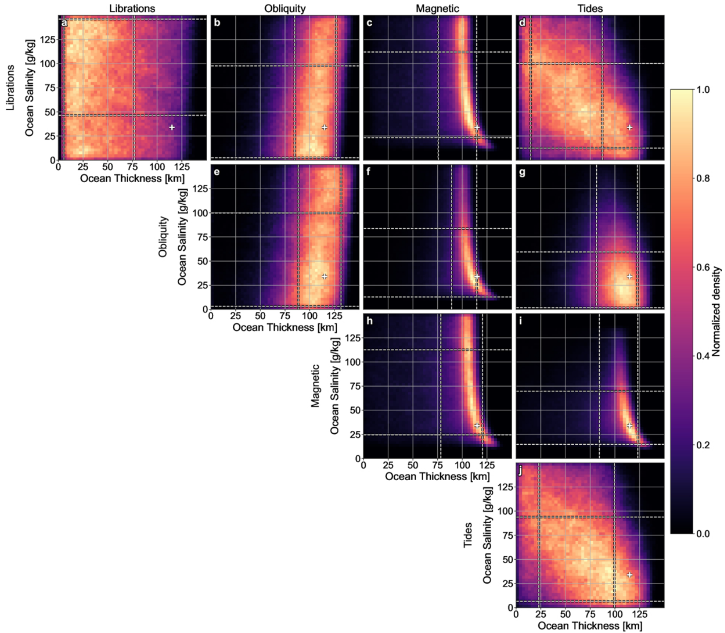
Figure 7. from Flavio Petricca et al 2026 Planet. Sci. J. 7 doi:10.3847/PSJ/ae5225 https://dx.doi.org/10.3847/PSJ/ae5225 © 2026. The Author(s). Published by the American Astronomical Society.
