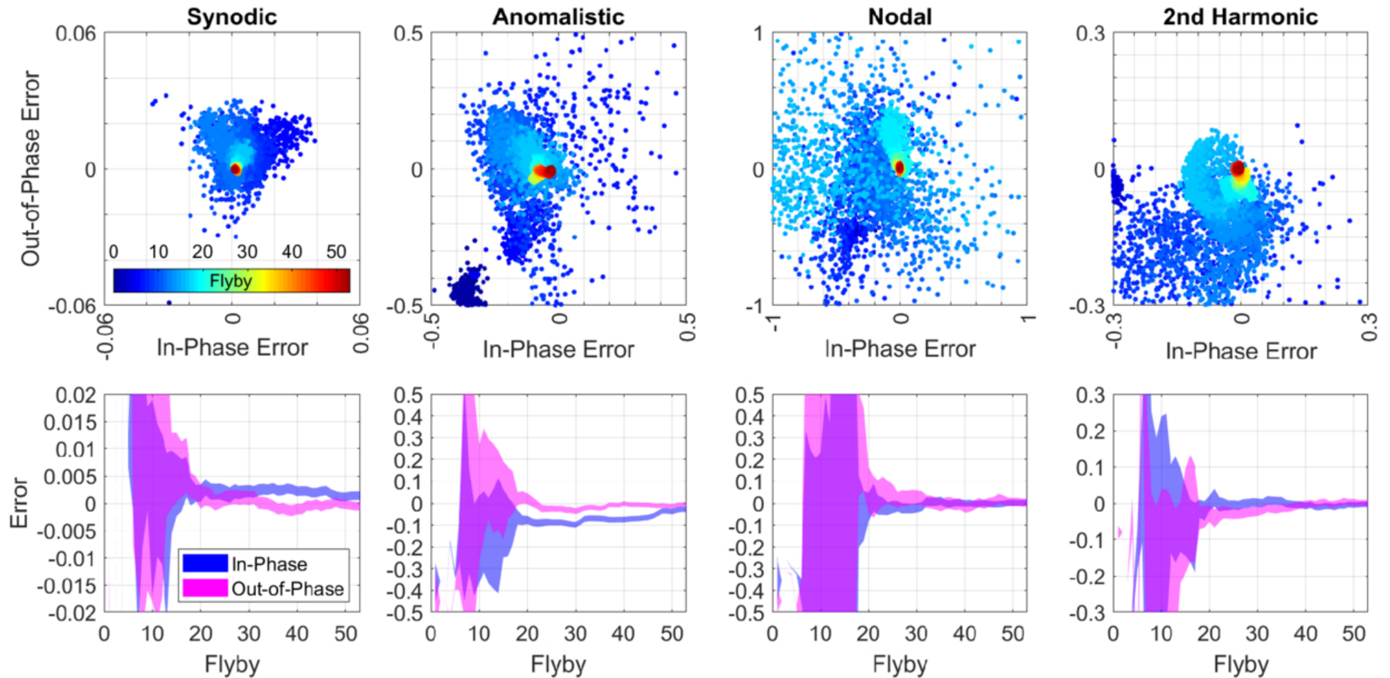
Figure 2. from Flavio Petricca et al 2026 Planet. Sci. J. 7 doi:10.3847/PSJ/ae5225 https://dx.doi.org/10.3847/PSJ/ae5225 © 2026. The Author(s). Published by the American Astronomical Society.
